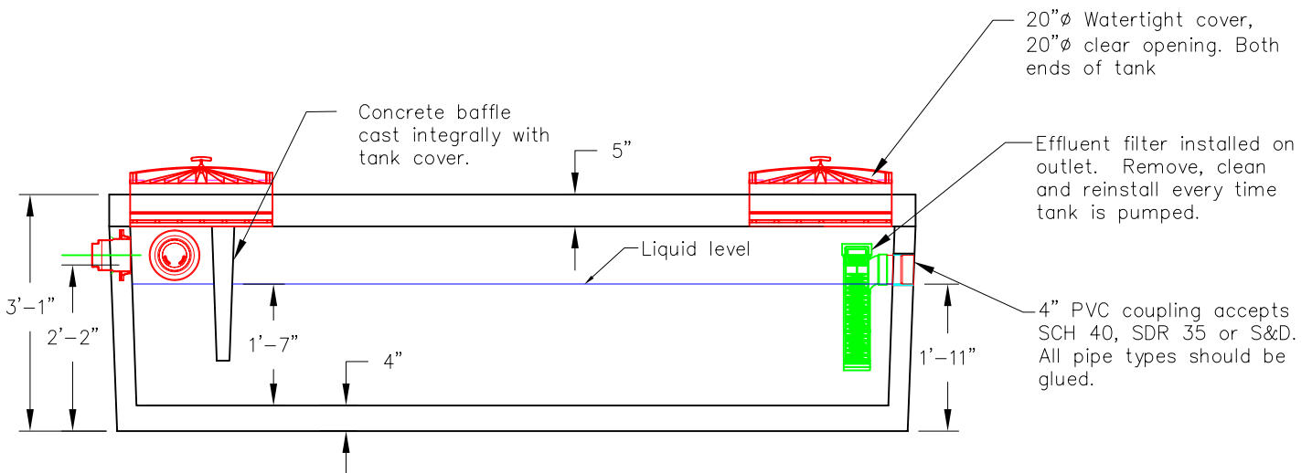
Section View
