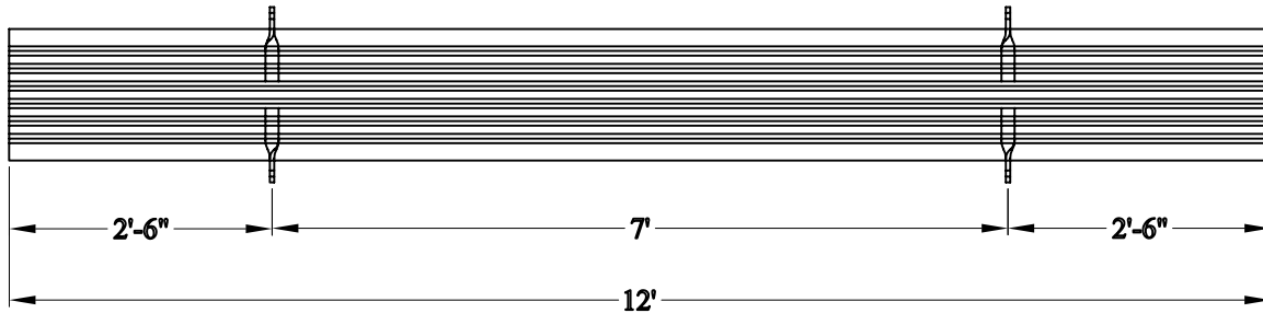
PLAN VIEW
